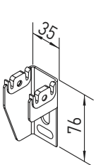
Bracket BP10/30
