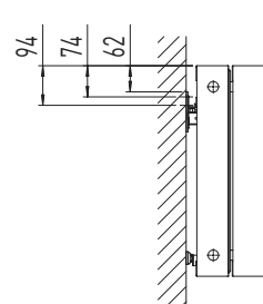
Plan double, profile
