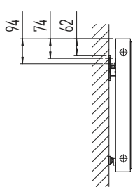
Plan single, profile
