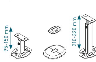
Adjustable console feet PR
